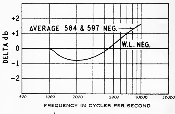
FIG. 12. Net improvement in high-frequency response of prints of ultraviolet negative over that of white-light negative.
